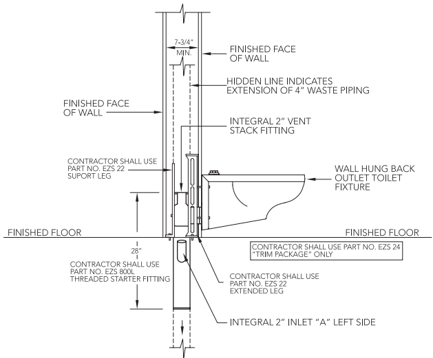
LEFT HAND FITTING - LEFT SIDE ELEVATION
