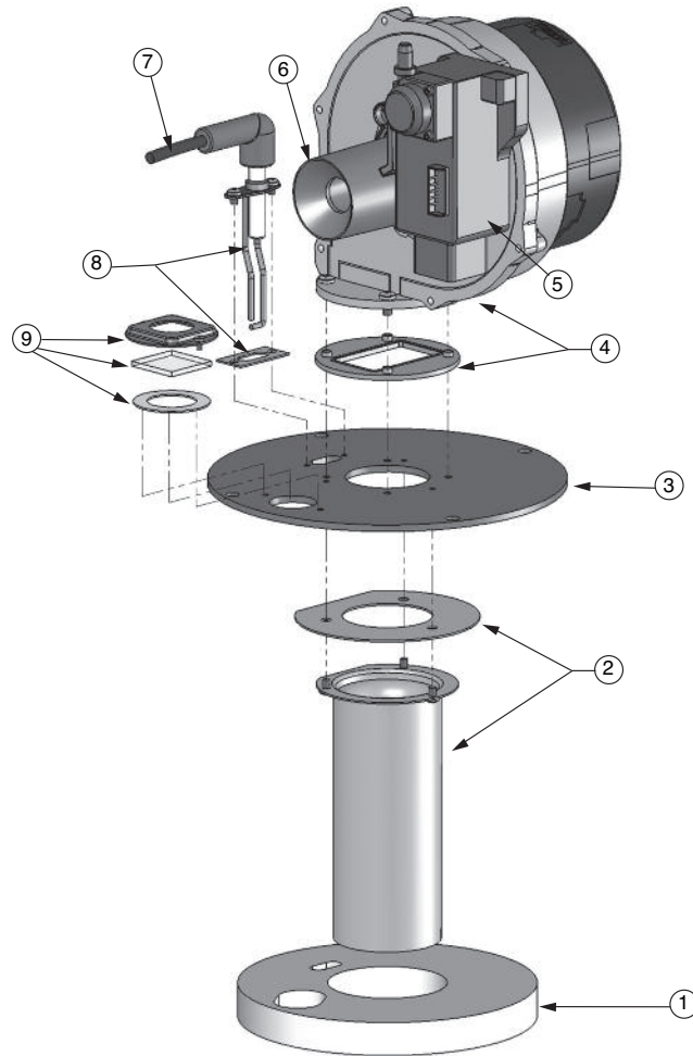
PRESTIGE Solo 60/175/250 Burner Components
